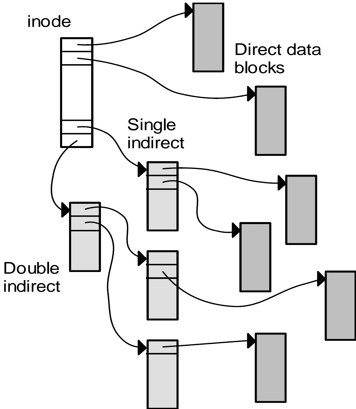
Figure 7. Inode as a data directory
